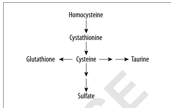
Figure 1. Transsulfuration pathway.
